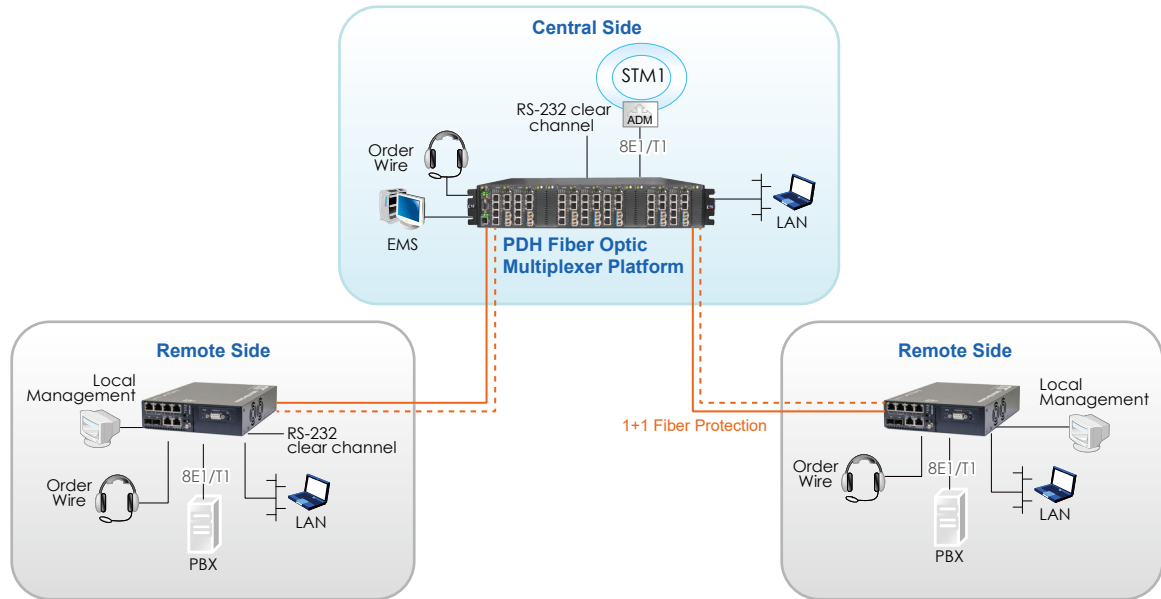
PDH Fiber Optical Multiplexer P2P Application
